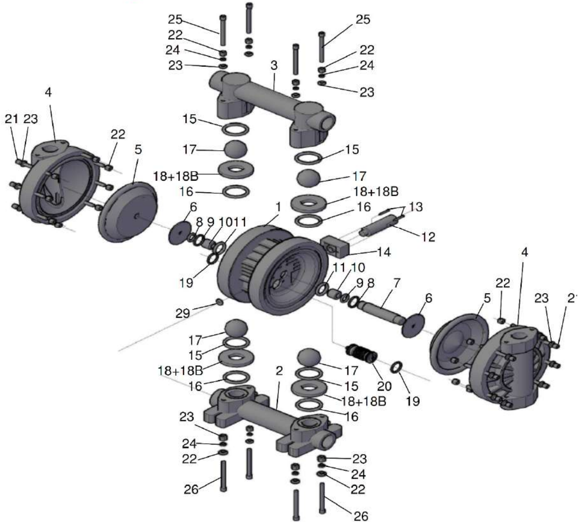
025 PP - PVDF spare part list pump
