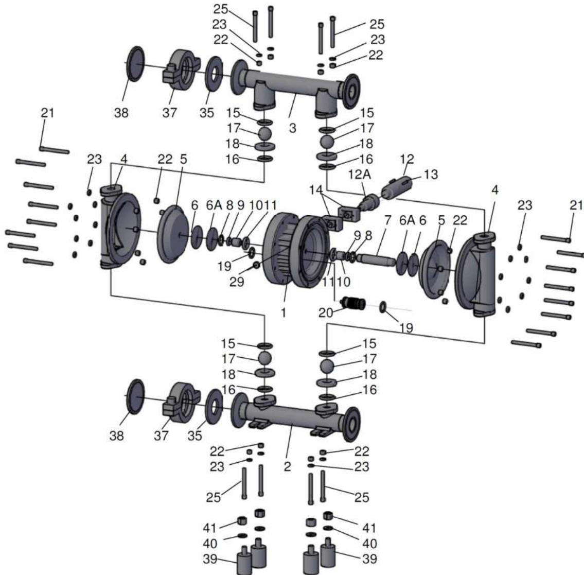
040 FDA Stainless steel spare part list pump
