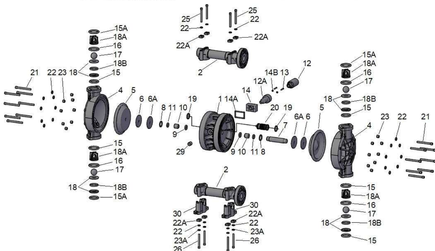
Spare Part list Drawing Ruby 141 Non Metallic
