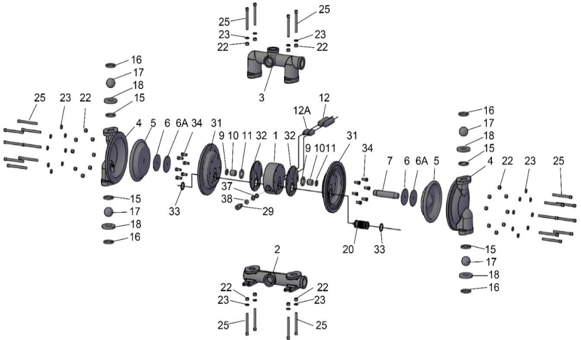
Spare Part List Drawing Ruby 140 AISI 316 with Metallic Center Block
