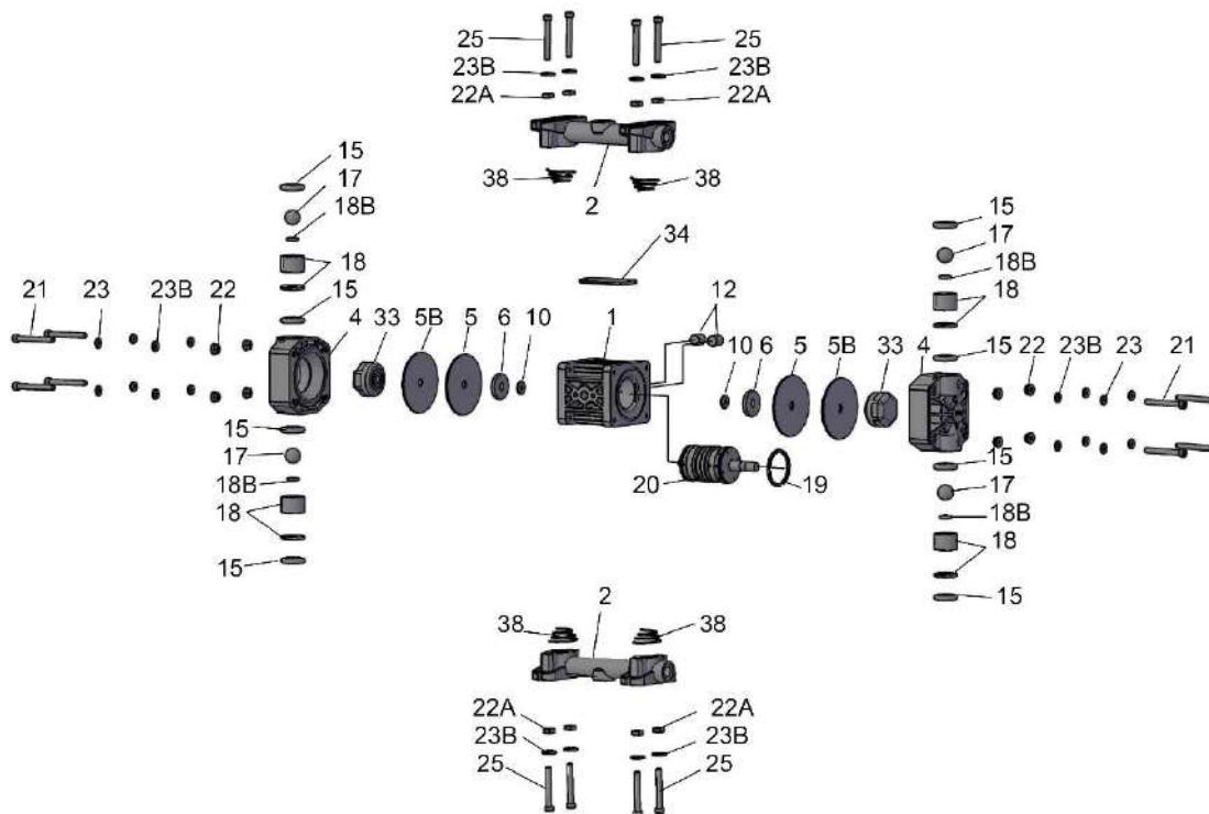
Spare Part List Drawing Ruby 008 Non Metallic
