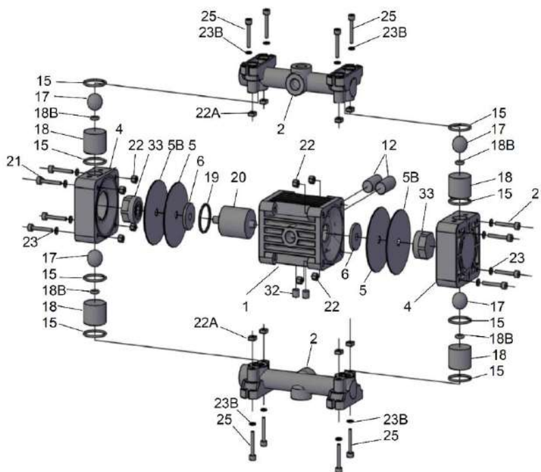
Spare Part List Drawing Ruby 010 Non Metallic
