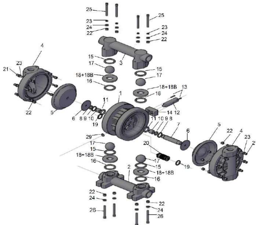
Spare Part List Drawing Ruby 025 Non Metallic
