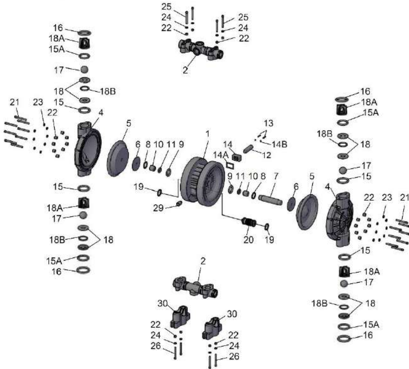
Spare Part List Drawing Ruby 125 Non Metallic
